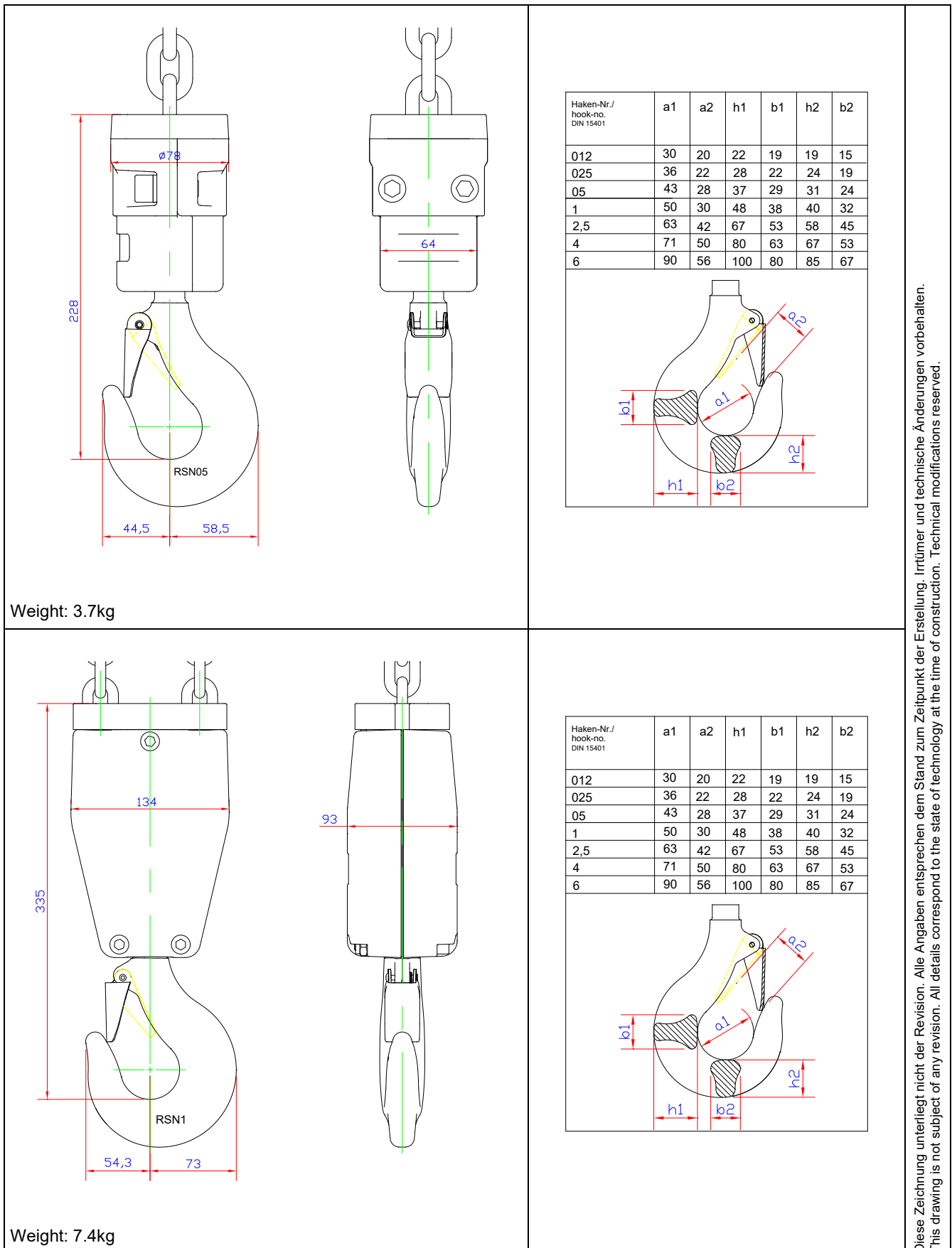
Figure 3 Hook tackle & hook block
